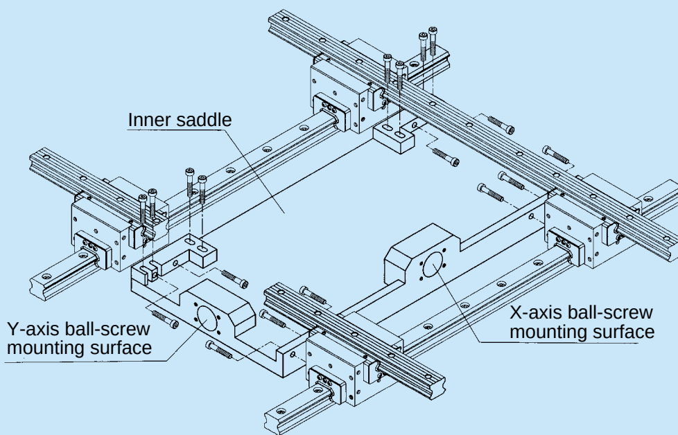
Inner saddle (with adjustment mechanism)
