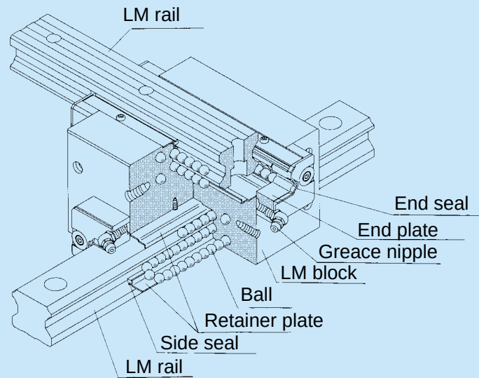
Fig. 1 Construction of Model CSR
