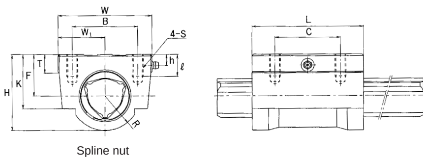
Spline nut
