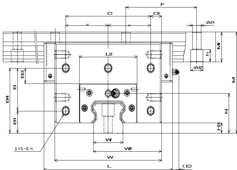
Outer dimensions
